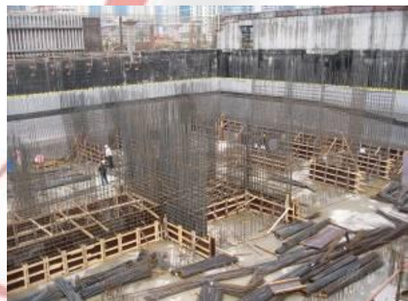
Reinforcement installation Wind Tower II
